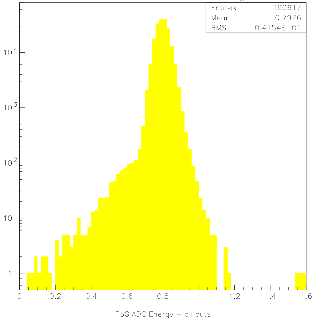
CKM Jlab Test Beam Data – PBG block Energy
