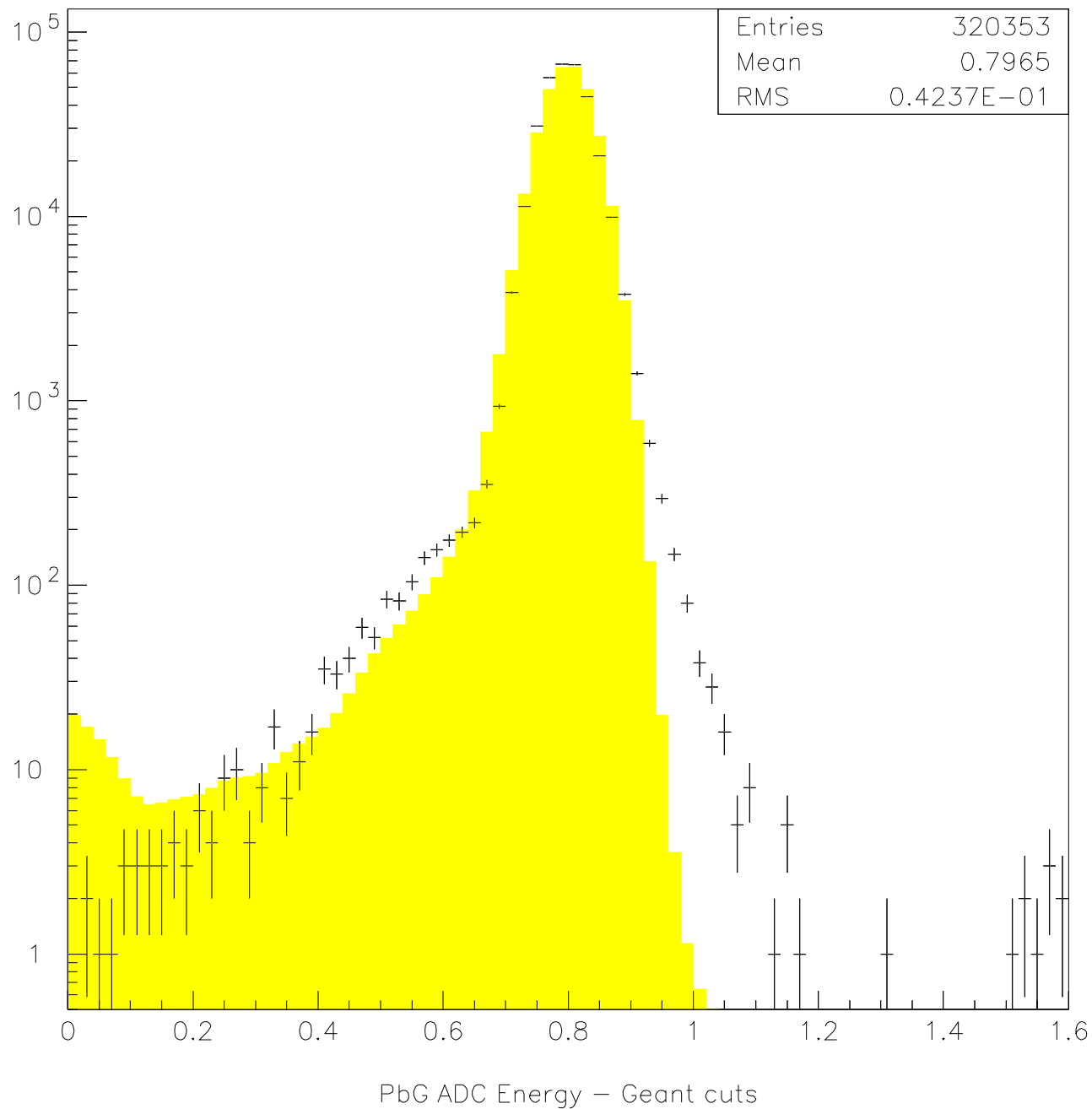
CKM PBG data and resolution smeared, rescaled, GEANT simulation
